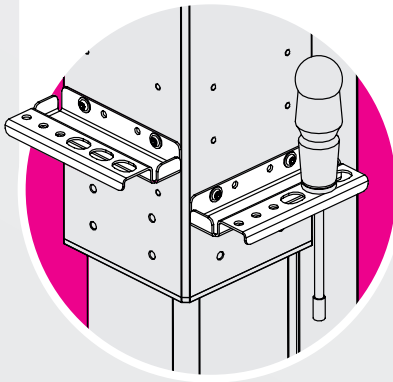
Tool holders
